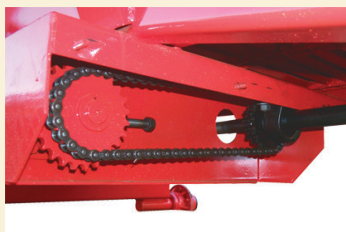
Microdoser Has 1:1 gear transmission to work with a double pulley or 1:2 with simple pulley. Maintains distribution speed.
